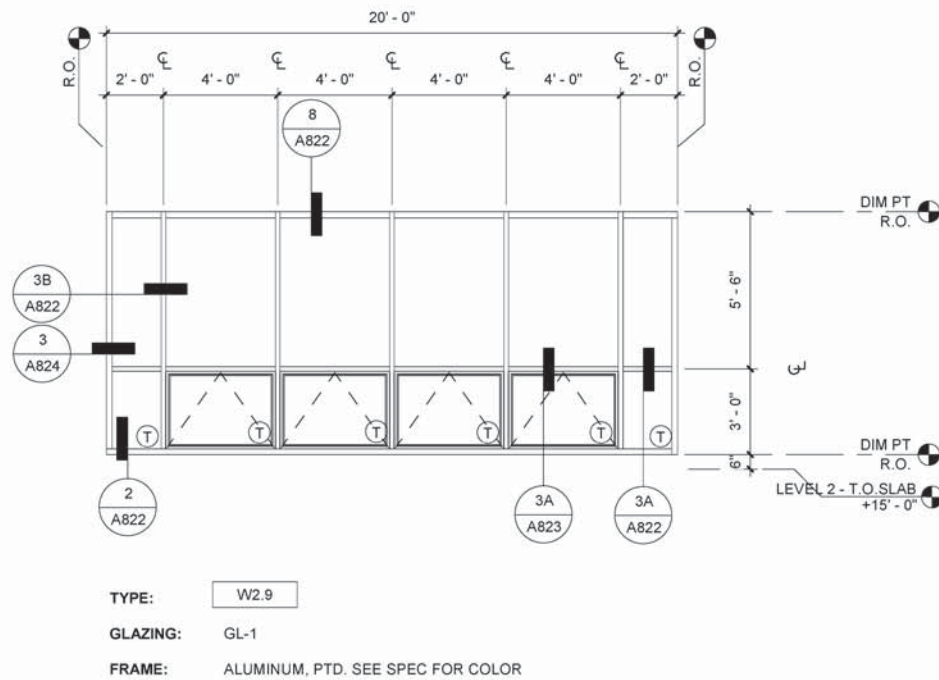
9 STOREFRONT W2.9 1/4" = 1'-0"
