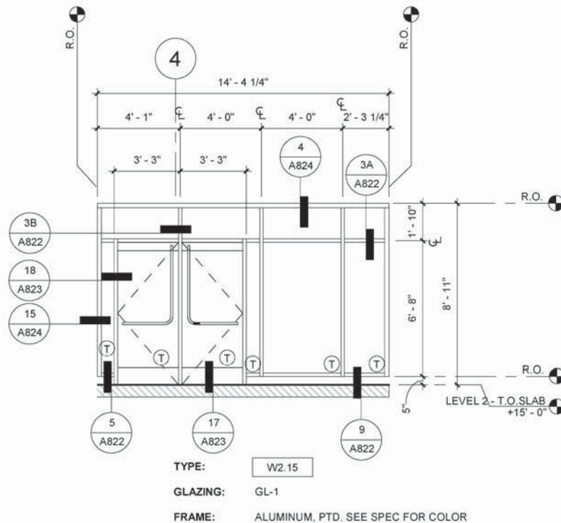
15 STOREFRONT W2.15 1/4" = 1'-0"
