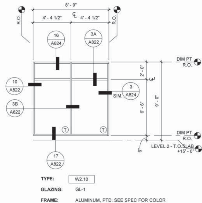
10 STOREFRONT W2.10 1/4" = 1'-0"
