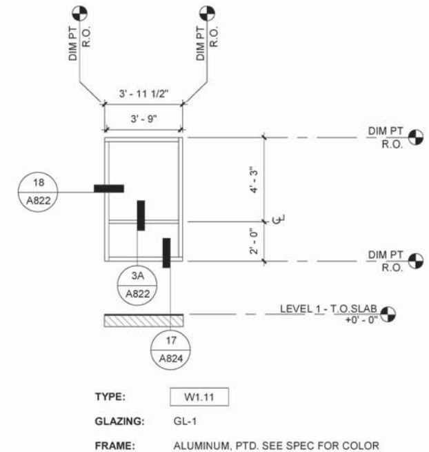
1 STOREFRONT W1.11 1/4" = 1'-0"
