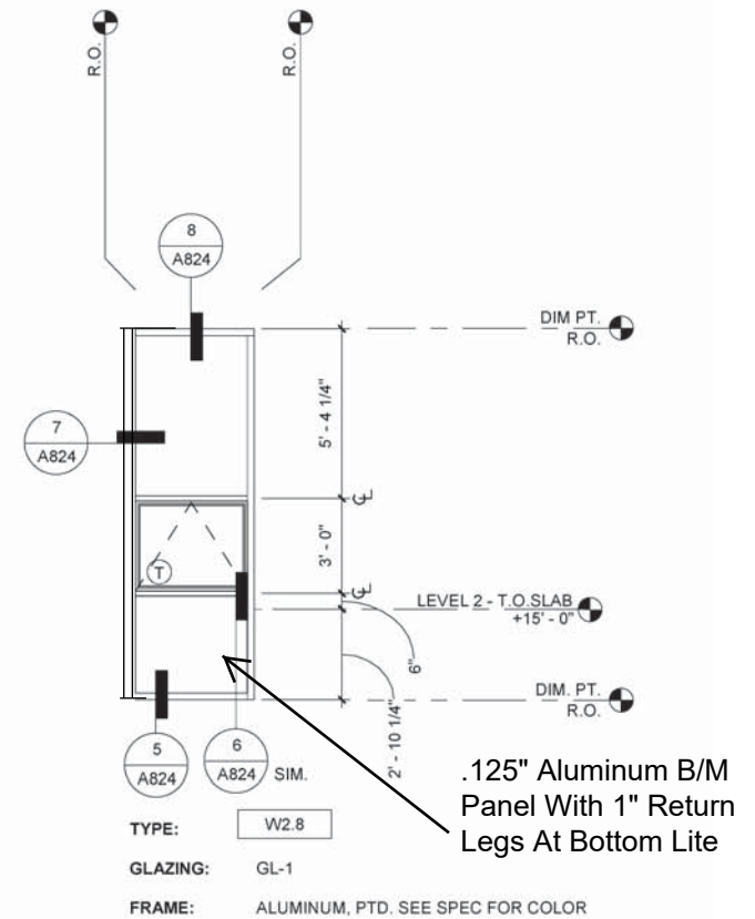
8 STOREFRONT W2.8 1/4" = 1'-0"
