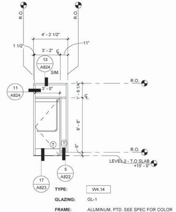
14 STOREFRONT W2.14 1/4" = 1'-0"
