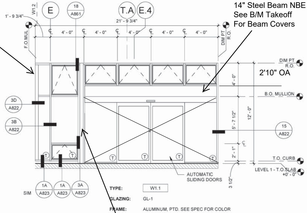
1 STOREFRONT W1.1 1/4" = 1'-0"
