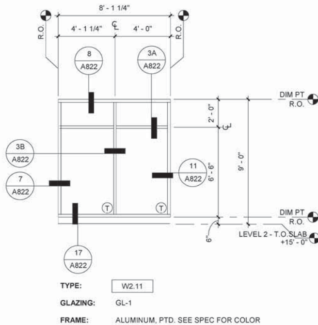
11 STOREFRONT W2.11 1/4" = 1'-0"
