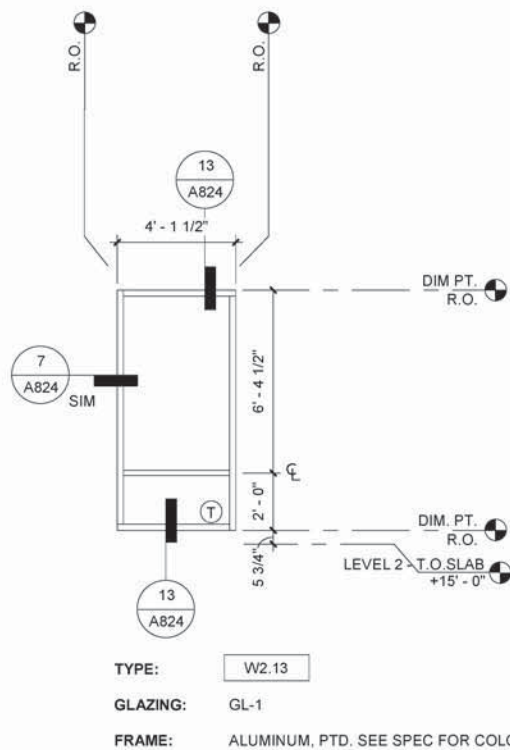
13 STOREFRONT W2.13 1/4" = 1'-0"
