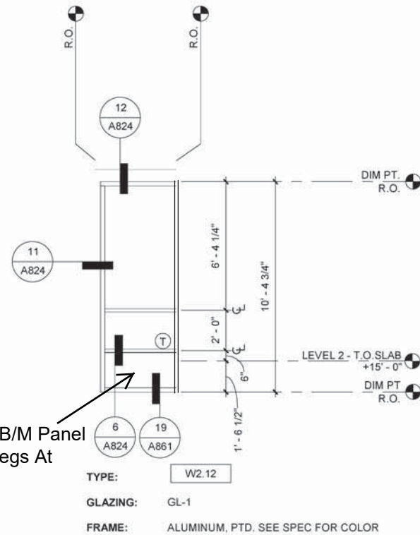
12 STOREFRONT W2.12 1/4" = 1'-0"
