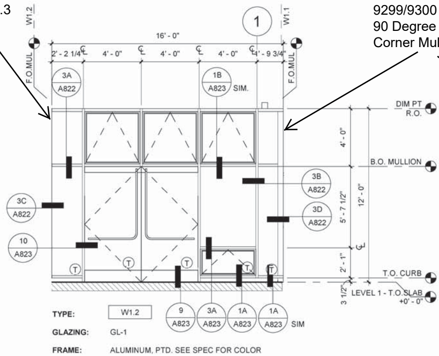
2 STOREFRONT W1.2 1/4" = 1'-0"
