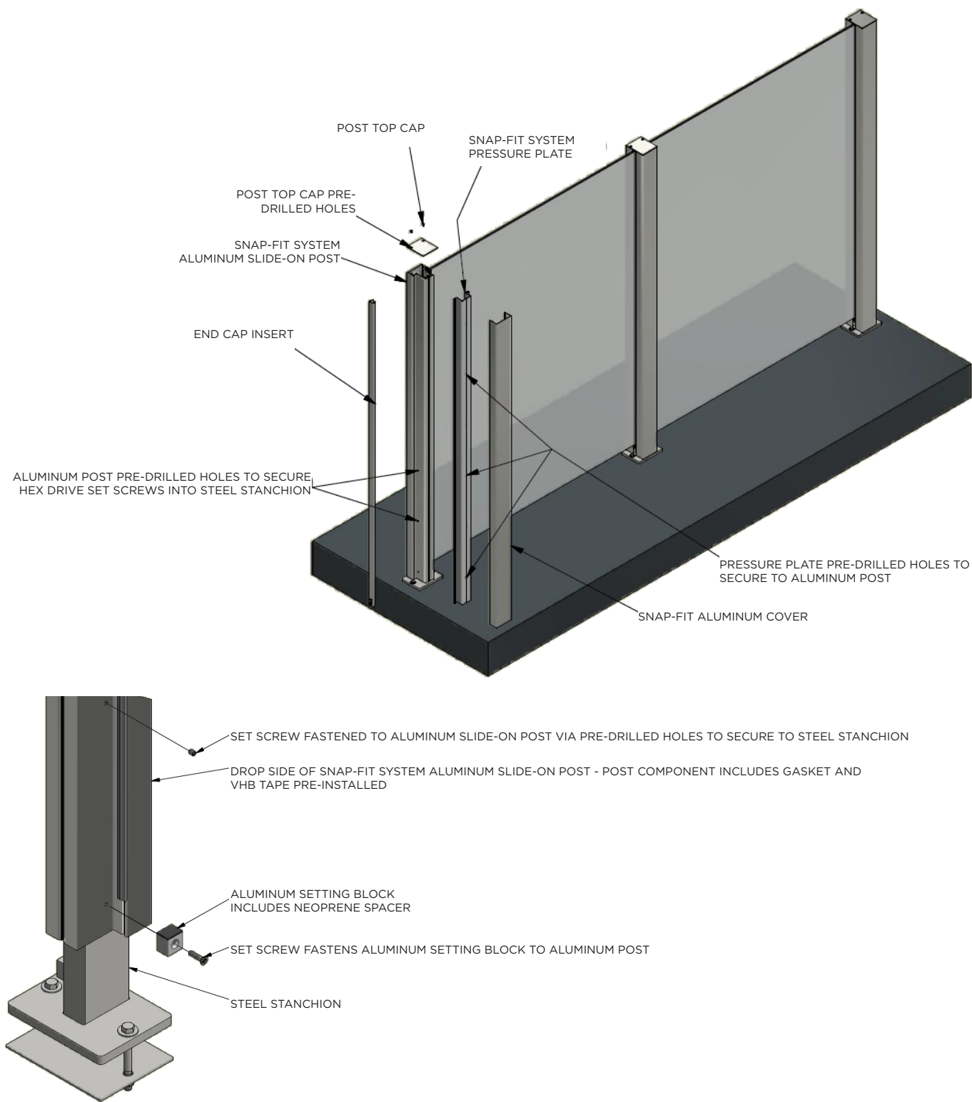
SET SCREW AND SETTING BLOCK ATTACHMENT DETAIL
